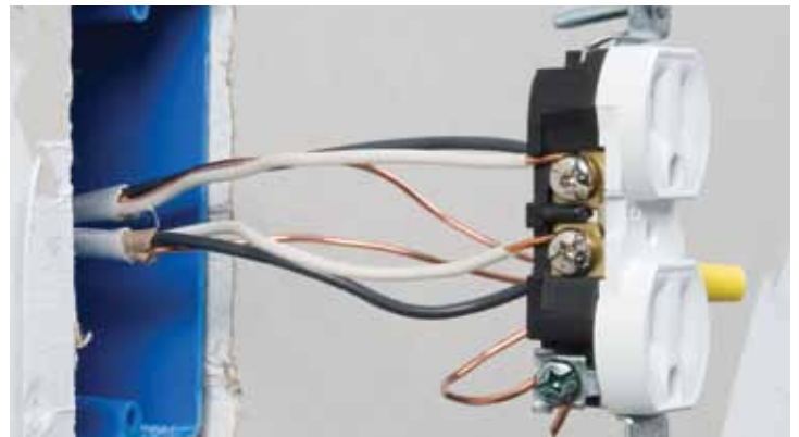
Photo 3: Wired receptacle not yet pushed back into box.
