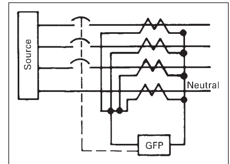
Figure 13. Schematic for Residual Method
