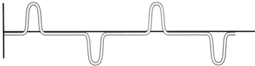
A Non-Linear Current and Its Fundamental, Plus 3rd and 5th Harmonic Components
